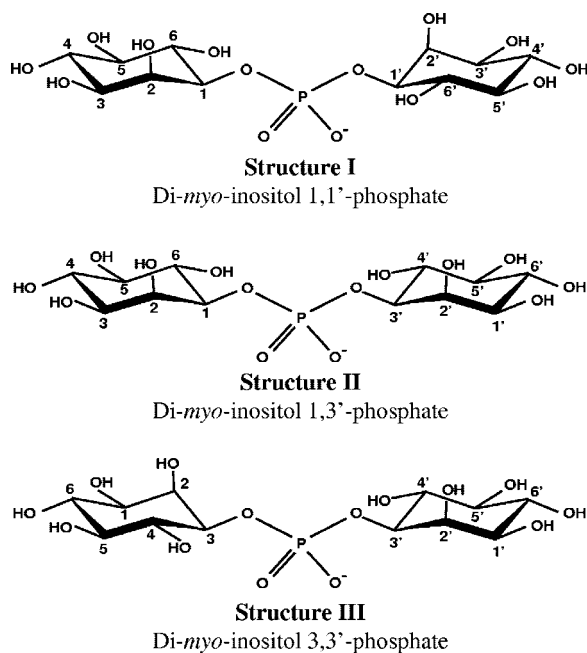
FIG. 1. The structures of the three possible stereoisomers of DIP. Structure I represents the configuration of DIP as reported by van Leeuwen et al. (30) and designated L,L-di- myo -inositol-1,1'-phosphate. Compounds I and III are stereoisomers, while compound II is optically inactive. In these representations, the numbering of the inositol atoms is based on the L configuration according to the "relaxation of lowest-locant rule" as recommended by the Nomenclature Committee of the International Union of Biochemistry in cases where metabolic relationships should be evidenced (20). A short note on myo -inositol nomenclature is given in the supplemental material.
